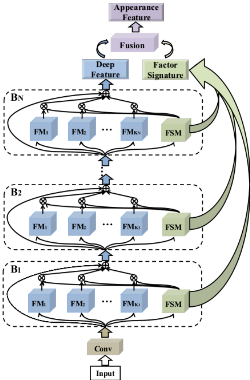
Figura 2.7: Multi-Level Factorisation Net (MLFN) . Reproduzida de [6]. ©2018 IEEE.
