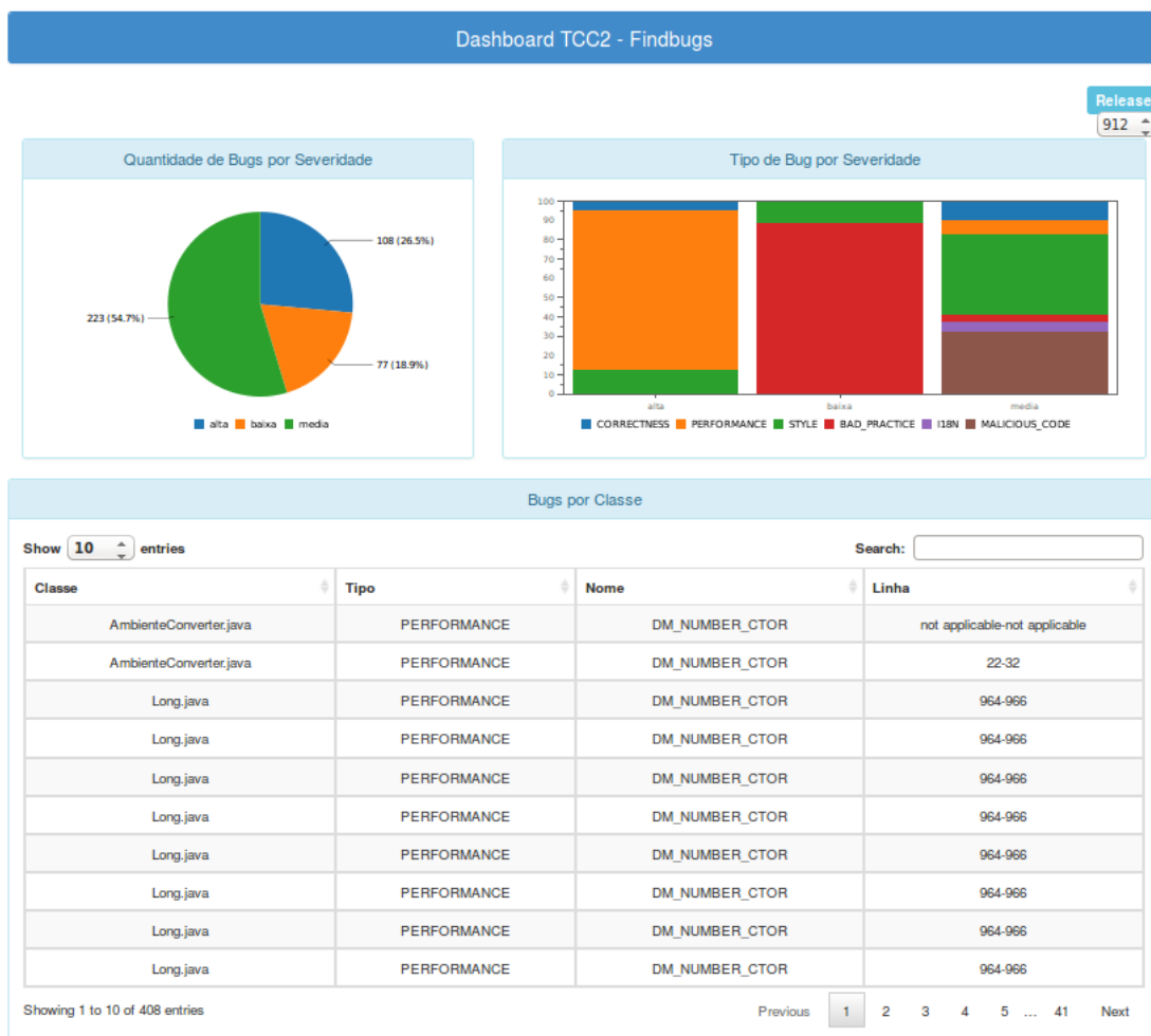
Figura 40 – Dashboard FindBugs
