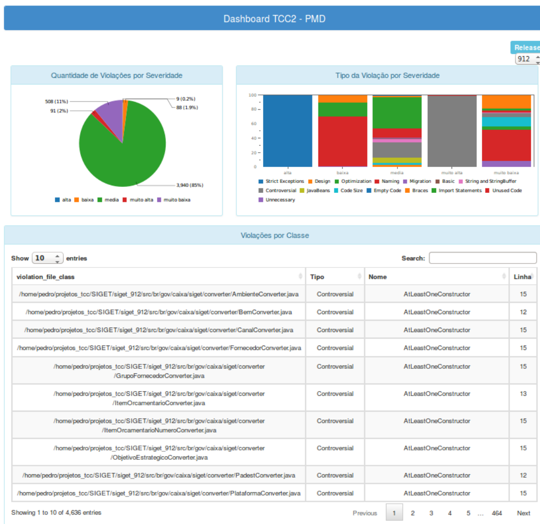
Figura 41 – Dashboard PMD
