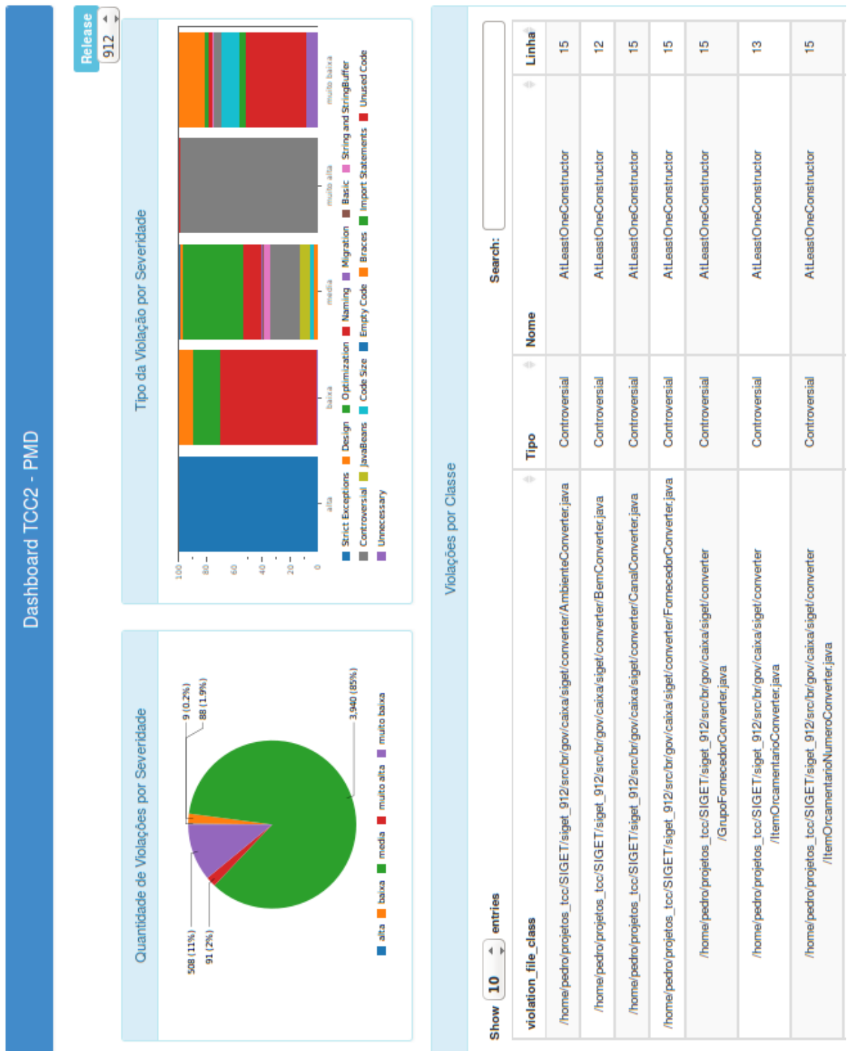
Figura 23 – Dashboard PMD
