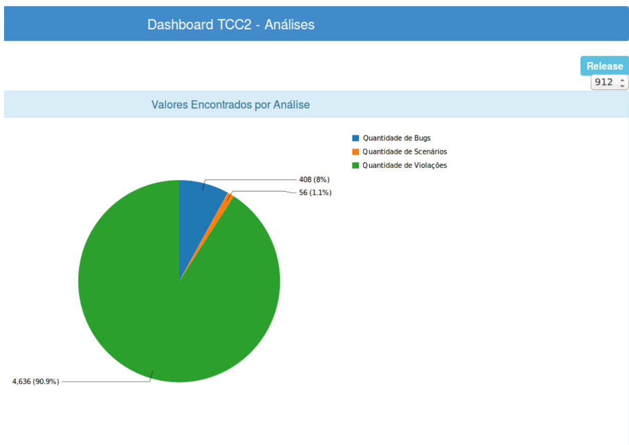
Figura 38 – Dashboard Geral
